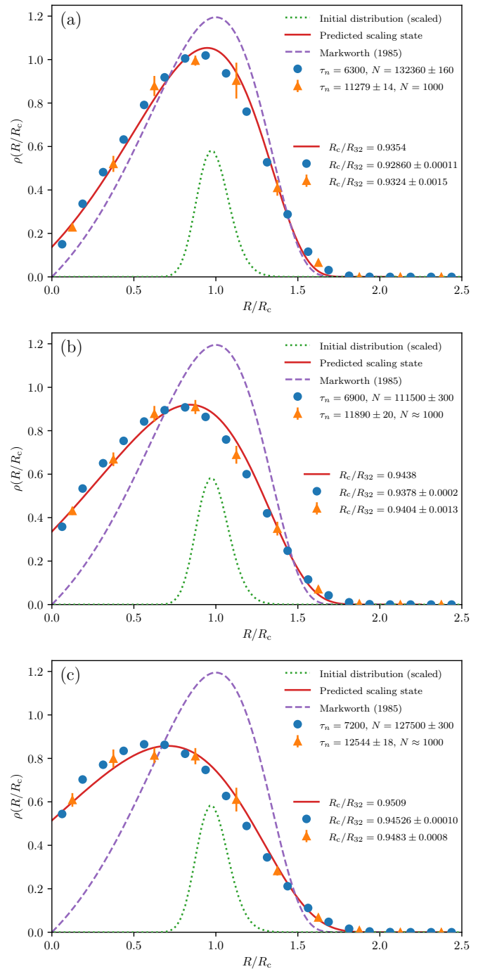
Fig. 6 Simulated bubble-size histograms for (a) \phi = 1\% , (b) \phi = 10\% , and (c) \phi = 35\% . The mean over five simulation runs is shown, and error bars give the sample standard deviation (where larger than the marker) over the five runs. The distributions are plotted when roughly N = 10^5 bubbles remain (with 20 bins), and when the runs halt (with 10 bins). The corresponding number \tau_n of completed time steps is given. The final N value is not exactly 10^3 because multiple bubbles can disappear in one time step. The uncertainties in the legend are due to differences between the five runs. Comparison is made to the predicted scaling state (27), and to that for the dry limit, the Lemlich-Markworth distribution (29). 12,36,46 The initial distribution (stated in the text) is also shown (not normalised, for clarity), as is the value of R_c/R_{32} for each histogram, alongside the theoretical prediction obtained as in figure 4.
