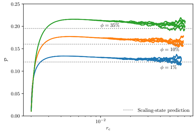
Fig. 10 Polydispersity 45 \mathcal{P} versus dimensionless critical radius, for various liquid fractions \phi . As in Figs. 6 and 8, the initial bubble-size distribution is lognormal with \sigma_R = 1/10 . Five runs per \phi are plotted, and the curves start after ten time steps. Comparison is made with the prediction of \mathcal{P} in the scaling state for each plotted \phi , which is obtained from the definition \mathcal{P} = R_{32}/\langle R^3 \rangle^{1/3} - 1 and the scaling-state distribution (27) by numerical integration.
