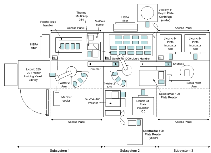
Fig. 1. Plan of our new Robot Scientist
